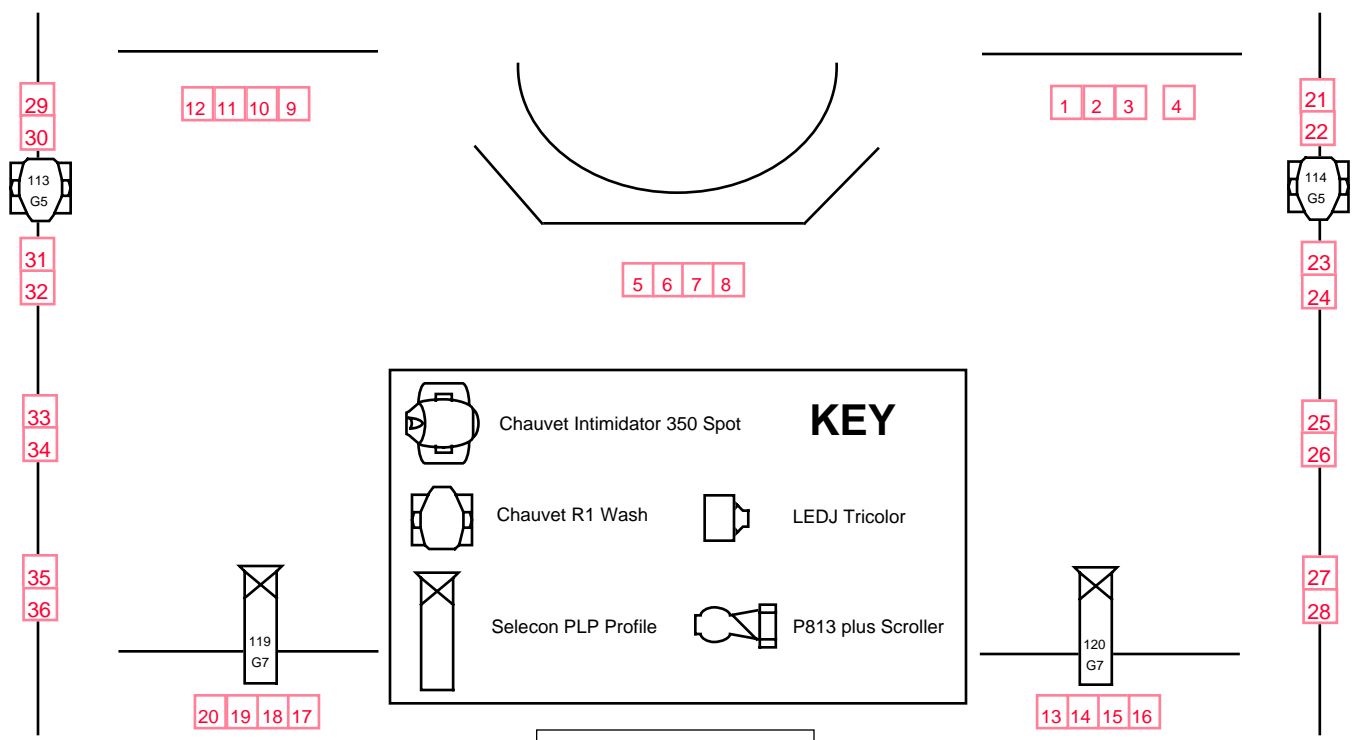
LED Rig Plan (Not to scale)
